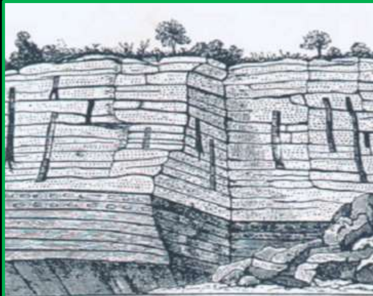
vertical trees in the Coal Measures sandstone, St.-Étienne, F Credner's Elemente der Geologie .
